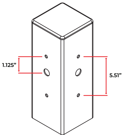
SQUARE POLE
