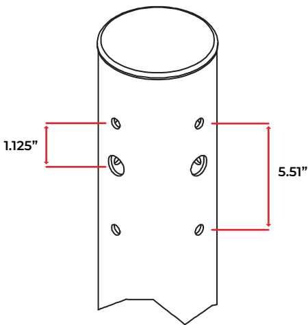
ROUND POLE
